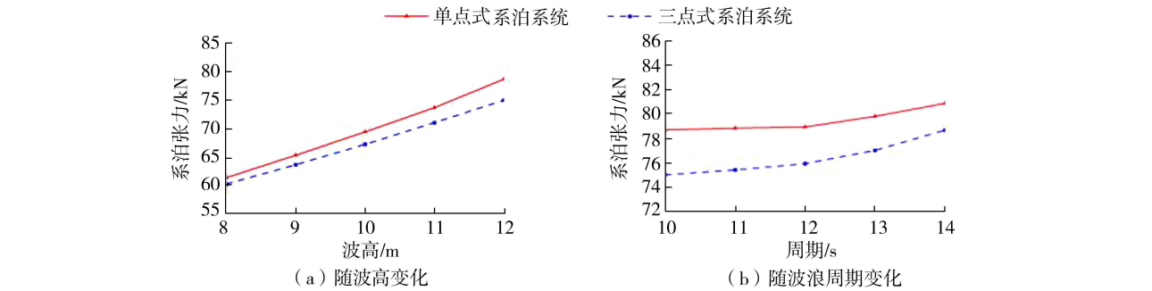
图 7 系泊张力最大值随波高与周期的变化曲线 Fig. 7 Variation of maximum mooring tension with different wave heights and periods
