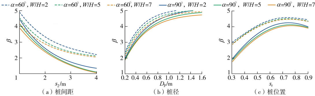
图 8 桩设计参数对桩加固边坡可靠度指标的影响 Fig. 8 Influence of pile design parameters on reliability index of pile-reinforced slope
