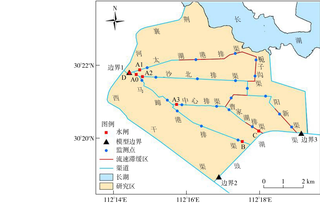
图 1 研究区水系及工程特征示意图 Fig. 1 Schematic diagram of river system and hydraulic structures in study area
