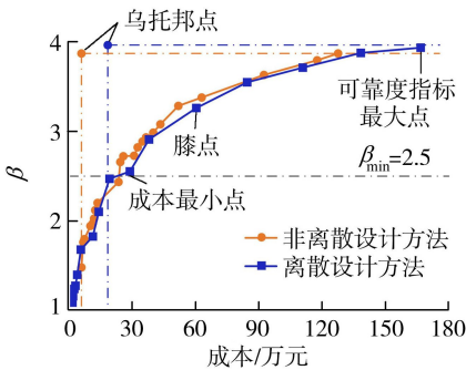
图 7 桩加固边坡设计的帕累托前沿 Fig. 7 Pareto front of pile-reinforced slope design
