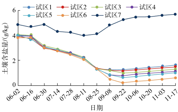
图2 0~20 cm 深度土壤含盐量变化曲线 Fig. 2 Variation of soil's salt content at a depth of 0-20 cm
