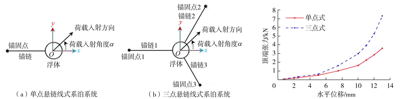
图 2 系泊系统坐标示意图 图 3 系泊系统静刚度曲线 Fig.2 Schematic diagram of mooring system coordinates Fig.3 Static stiffness curve of mooring system
