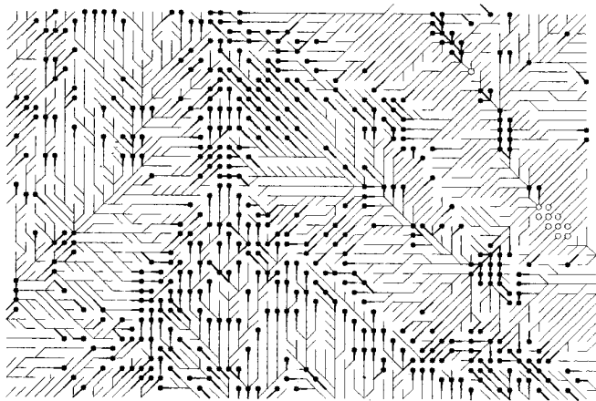
图8 流域D上由 30\text{ m}\times 30\text{ m} 的DEM导出的部分流水网 Fig.8 Part of drainage network derived according to the DEM of 30\text{ m}\times 30\text{ m} in catchment D
