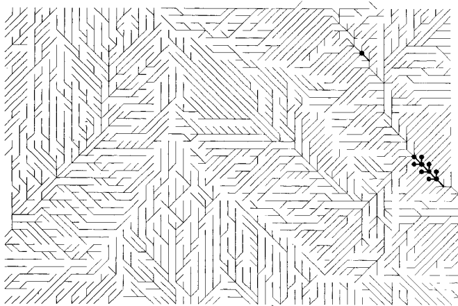
图9 流域D上由 30\text{ m}\times 30\text{ m} 的DEM导出的部分流水网(所示区域同图8) Fig.9 A part of drainage network derived according to the DEM of 30\text{ m}\times 30\text{ m} in catchment D (The display area is the same as that of Fig.8)
