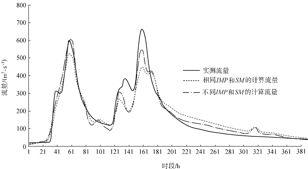
图 4 马道站 8404 次洪水过程线 Fig.4 Hourly discharge hydrograph for No.8404 flood event occurring at Madao station in 1984
