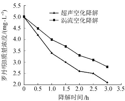
图 7 涡流空化和超声空化降解罗丹明 B Fig.7 Rhodamine B for swirling and ultrasonic cavitation degradations
