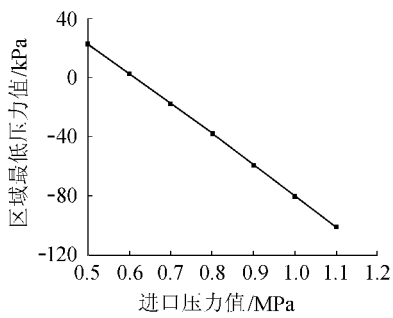
图 6 不同进口压力时区域最低压力分布曲线 Fig.6 Distribution of lowest pressure curves in the region with different inlet pressures
