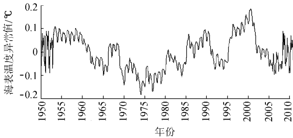
图3 月均海表温度距平3a低通滤波信号 Fig. 3 Monthly average SST anomaly after three-year low pass filter
